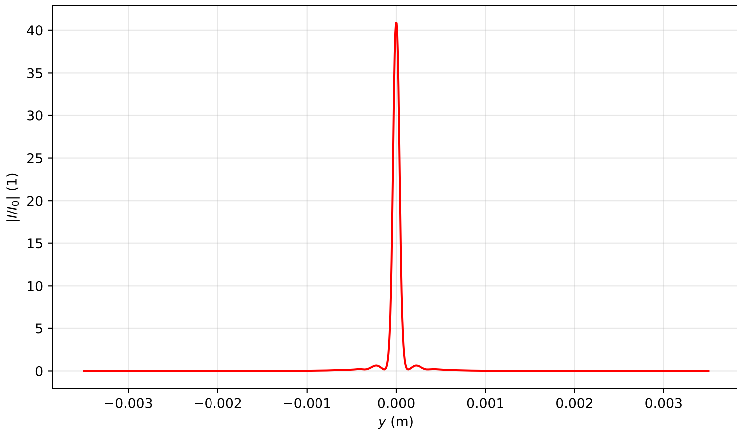
Intensity profile I(x=0, y, z=0.955)/I_0 , P_{in}=2.5P_{cr} , artificial time
